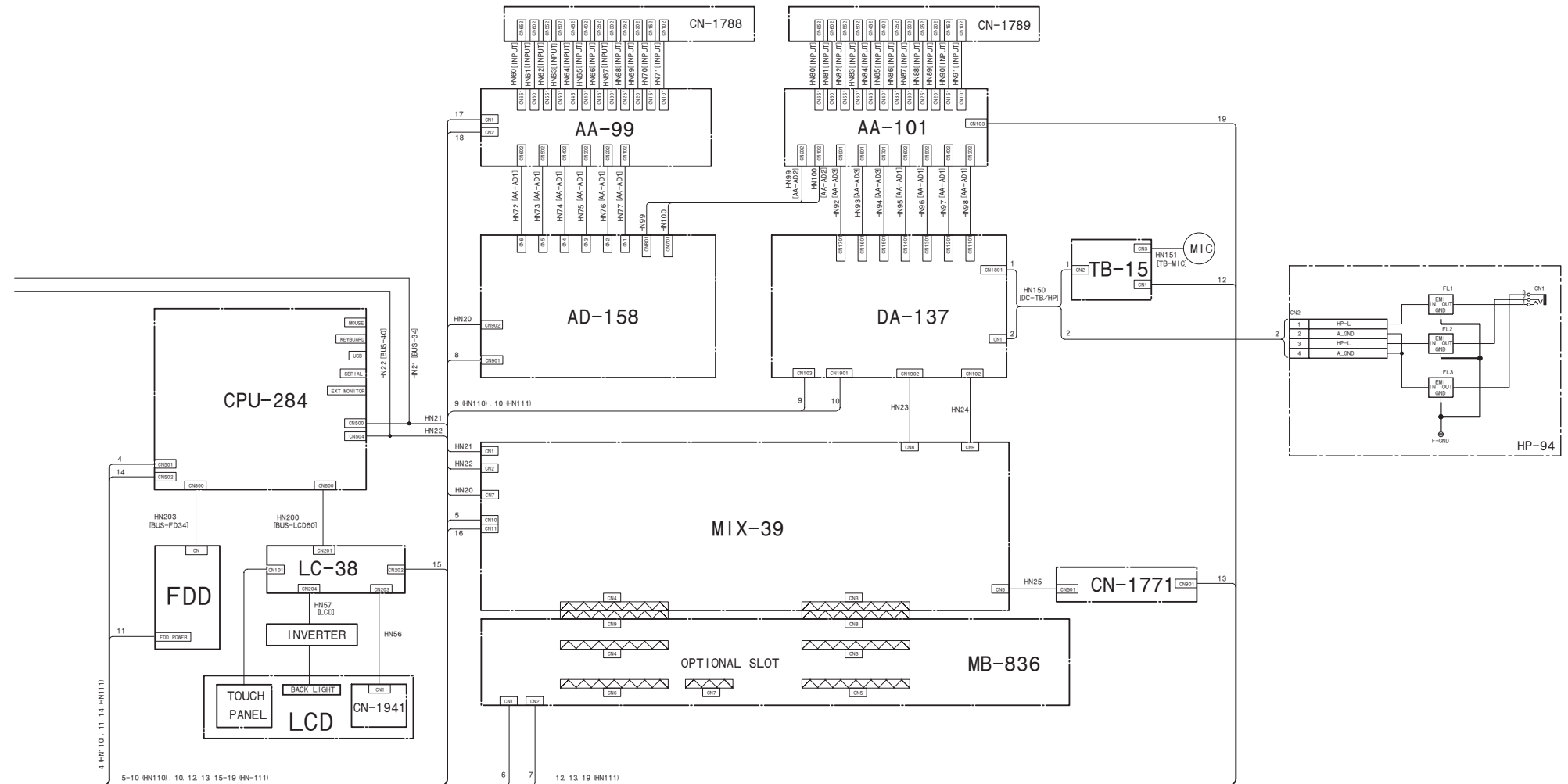
Frame Wiring GS-APX-397_FRAME_001_002 HP-94 BOARD NO. 1-675-880-12 GS-APX-397_HP-94_001_001
